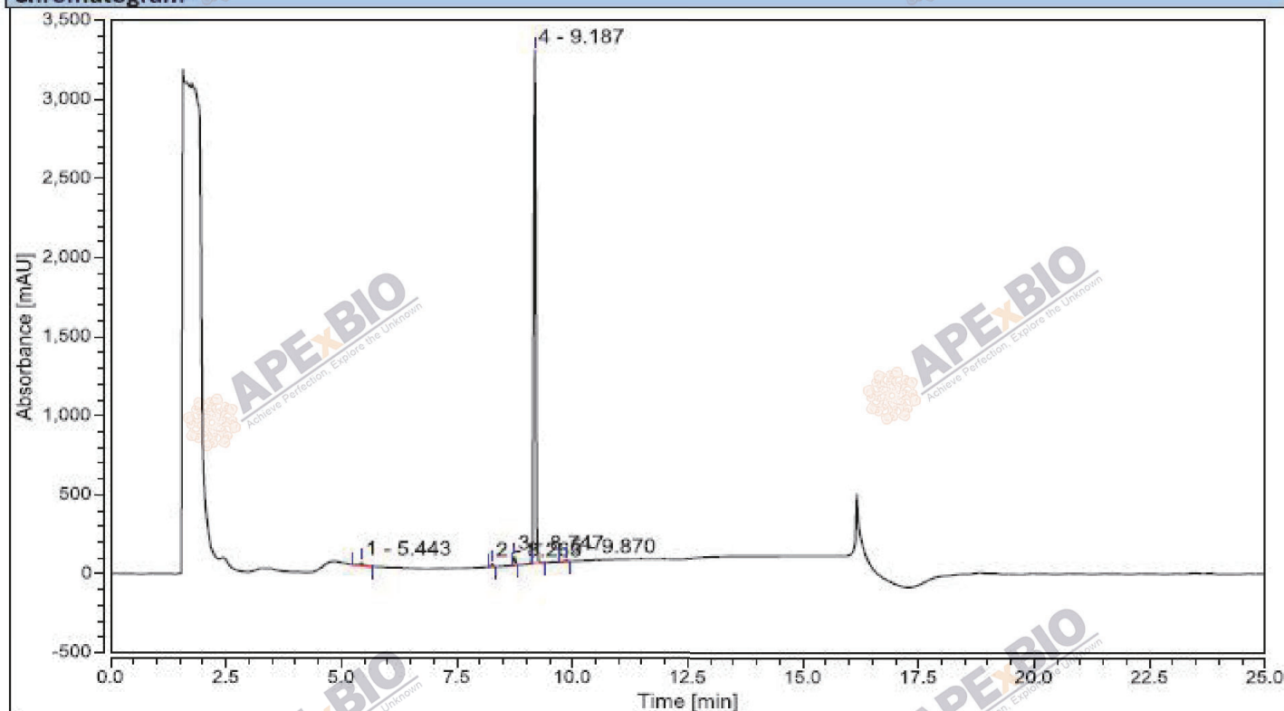
Chromatogram
