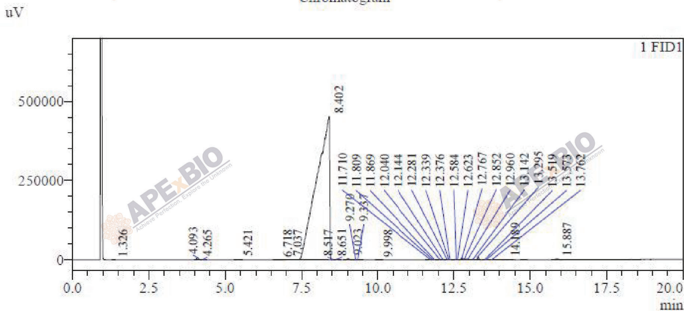
Chromatogram
