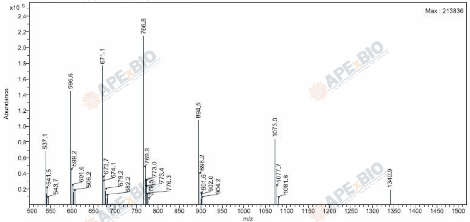
MS1 +Scan ESI (rt: 0.567 min) Frag=135V Gain=1.0
