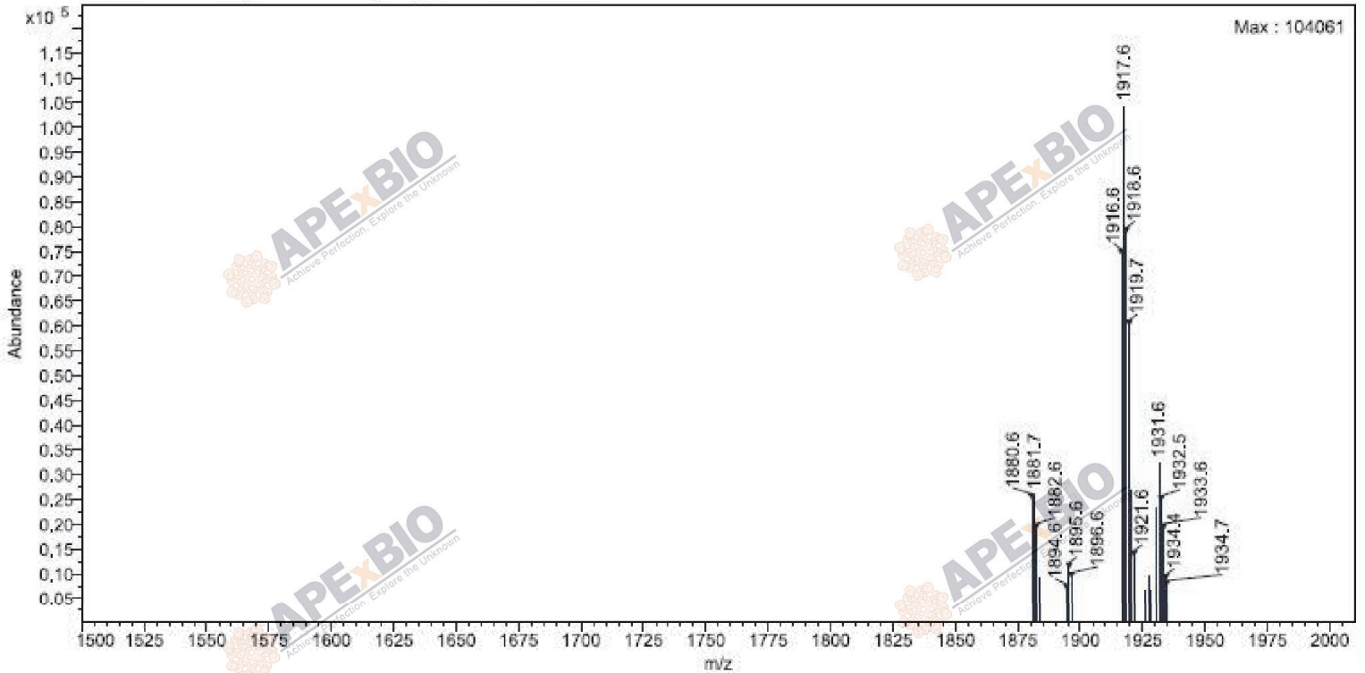
MS1 -Scan ESI (rt: 0.315 min) Frag=135V Gain=1.0
