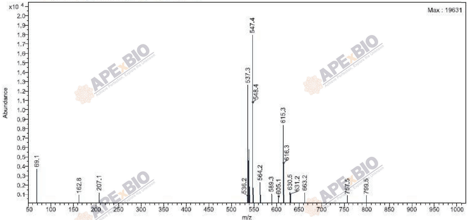
MS1 -Scan ESI (rt: 0,960 min) Frag=135V Gain=1,0
