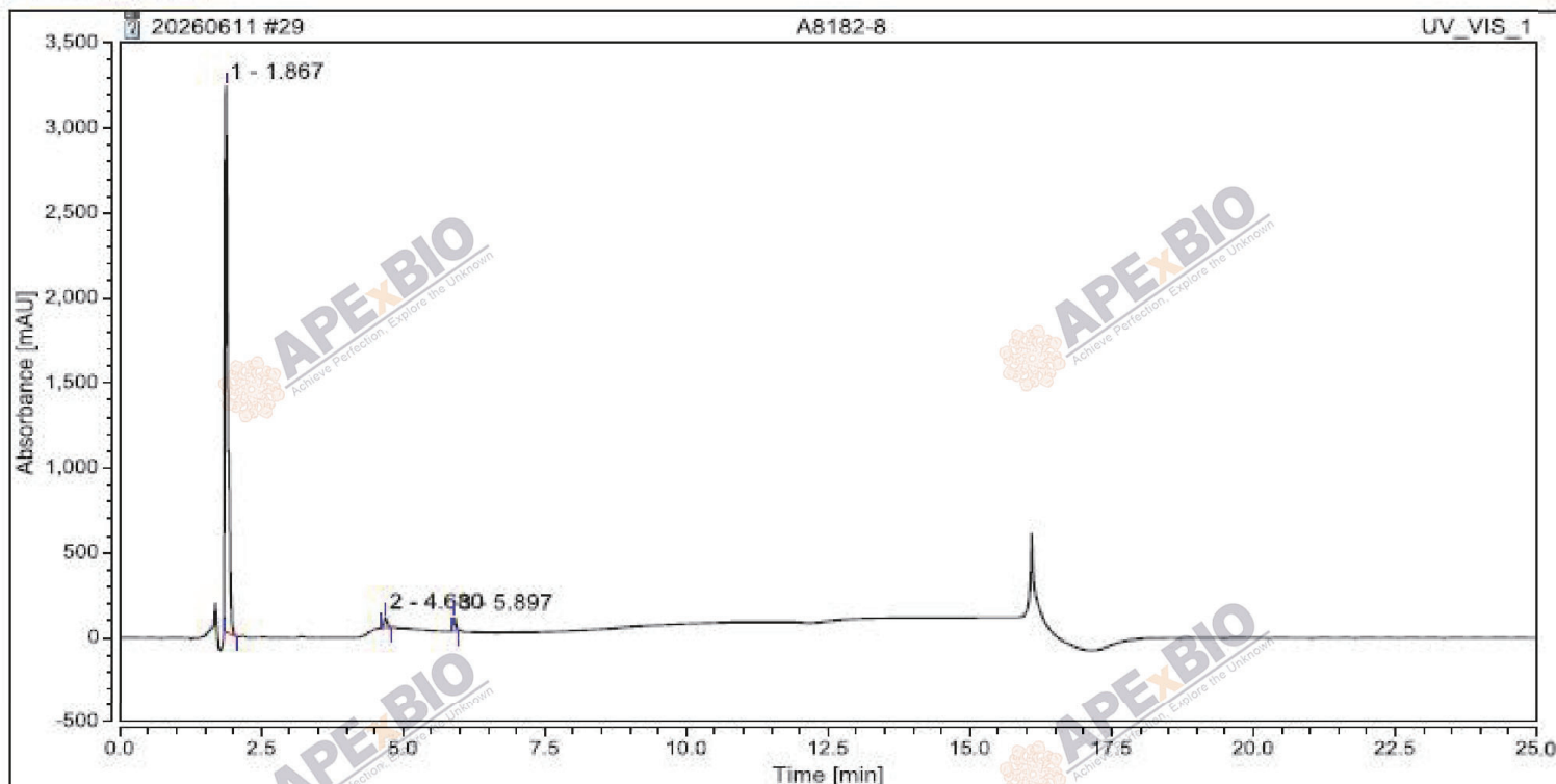
Chromatogram
