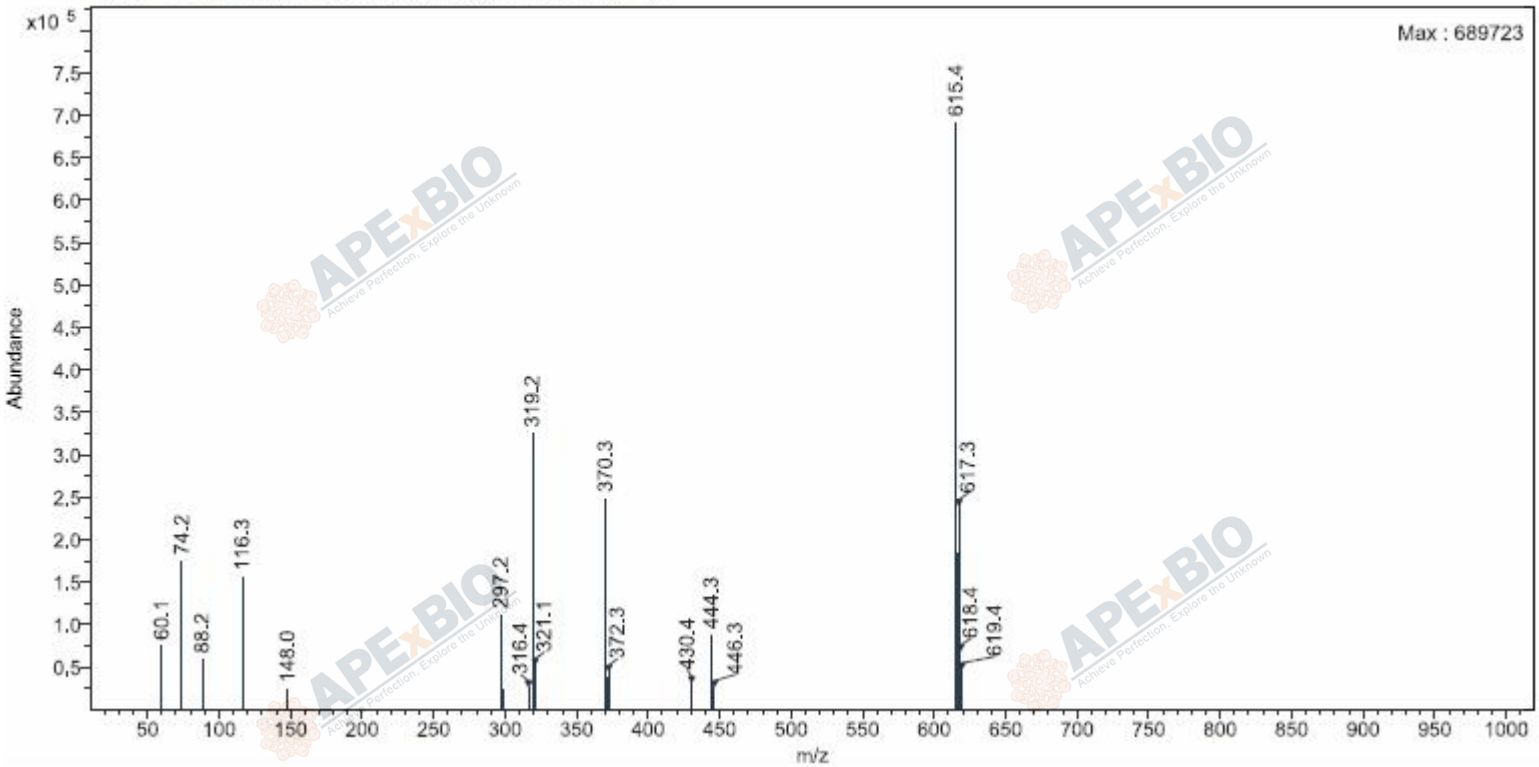
MS1 +Scan ESI (rt: 0,622 min) Frag=135V Gain=1,0
